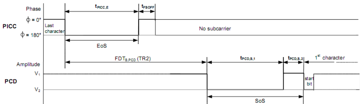
图20 FDT_{B,PCD}
