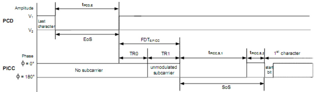
图16 FDT_{B,PICC}
