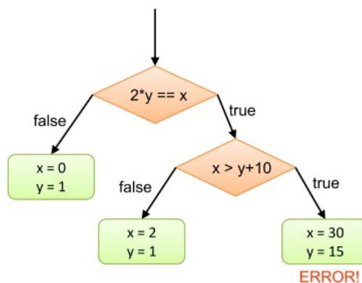
Figure 2. Execution tree for the example in Figure 1.
