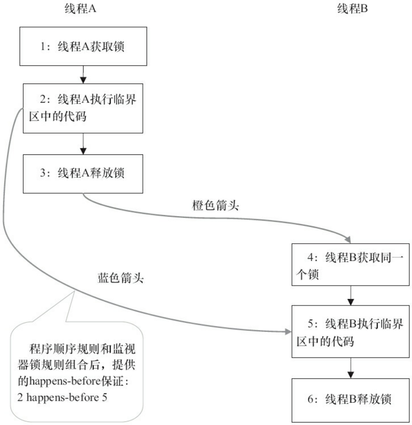
图3-24 happens-before关系图
