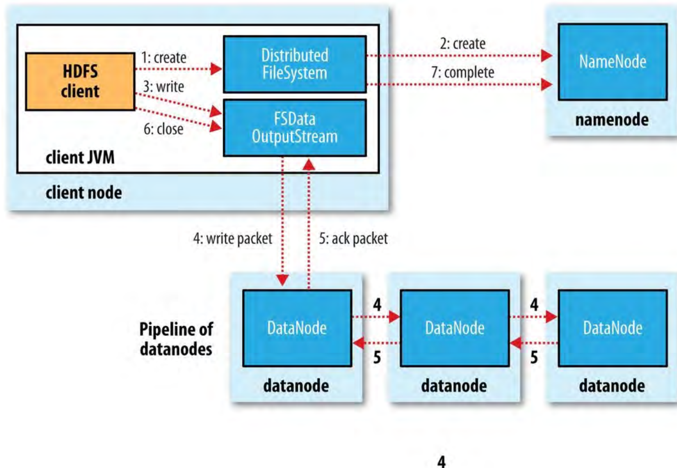
Figure 3-4. A client writing data to HDFS
