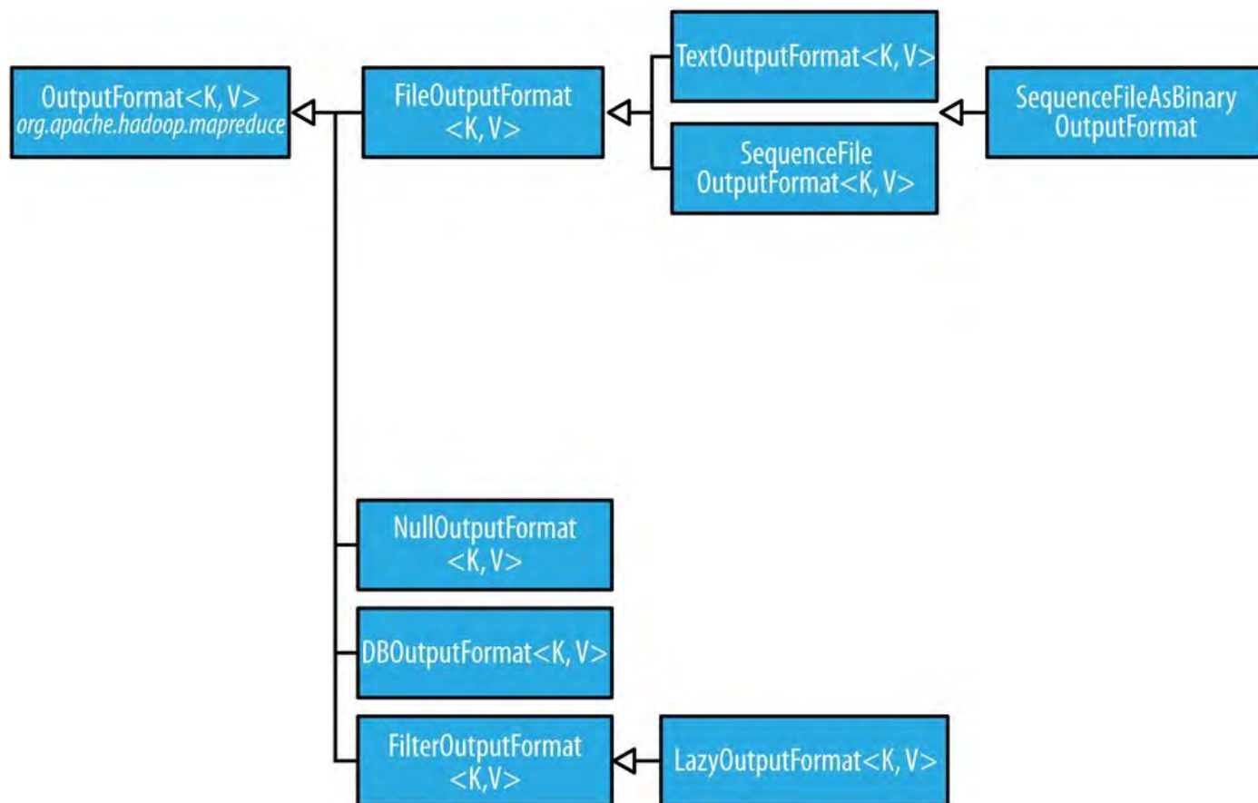
Figure 8-4. OutputFormat class hierarchy
