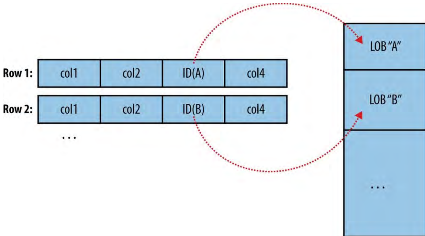
Figure 15-3. Large objects are usually held in a separate area of storage; the main row storage contains indirect references to the large objects
