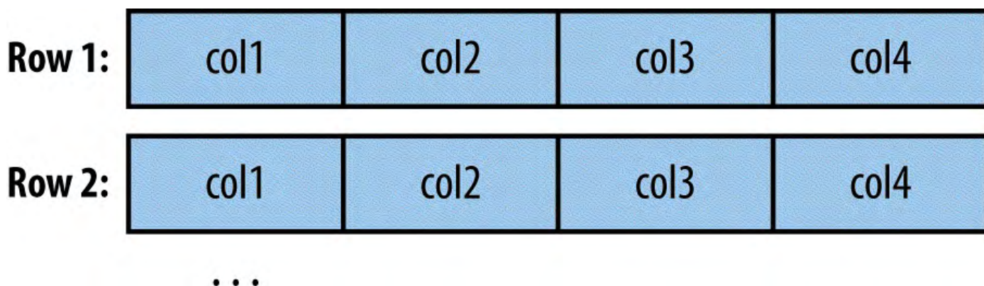
Figure 15-2. Database tables are typically physically represented as an array of rows, with all the columns in a row stored adjacent to one another
