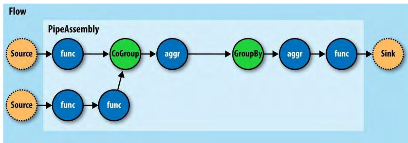
Figure 24-7. A Flow
