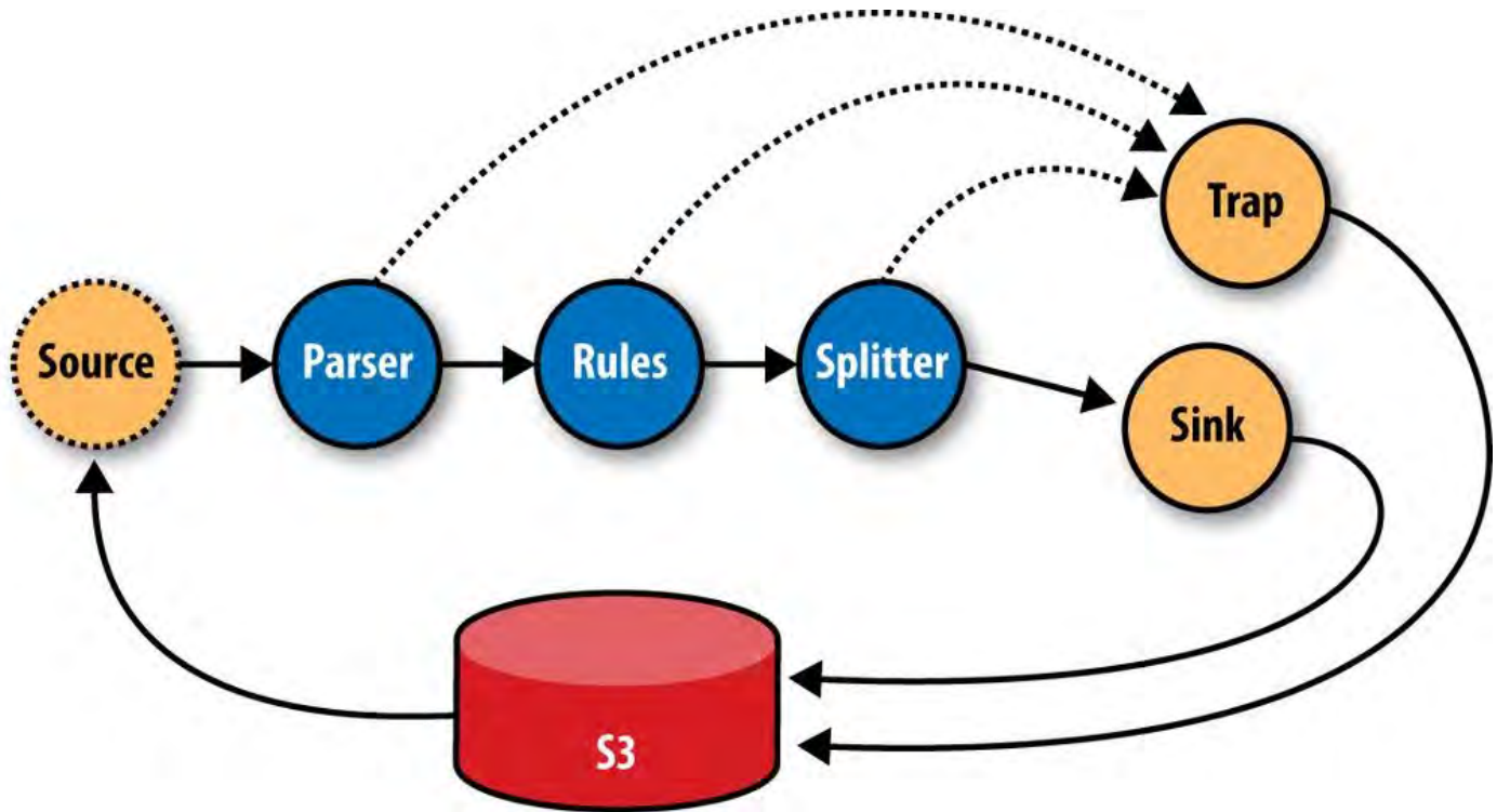
Figure 24-10. The ShareThis log processing flow
