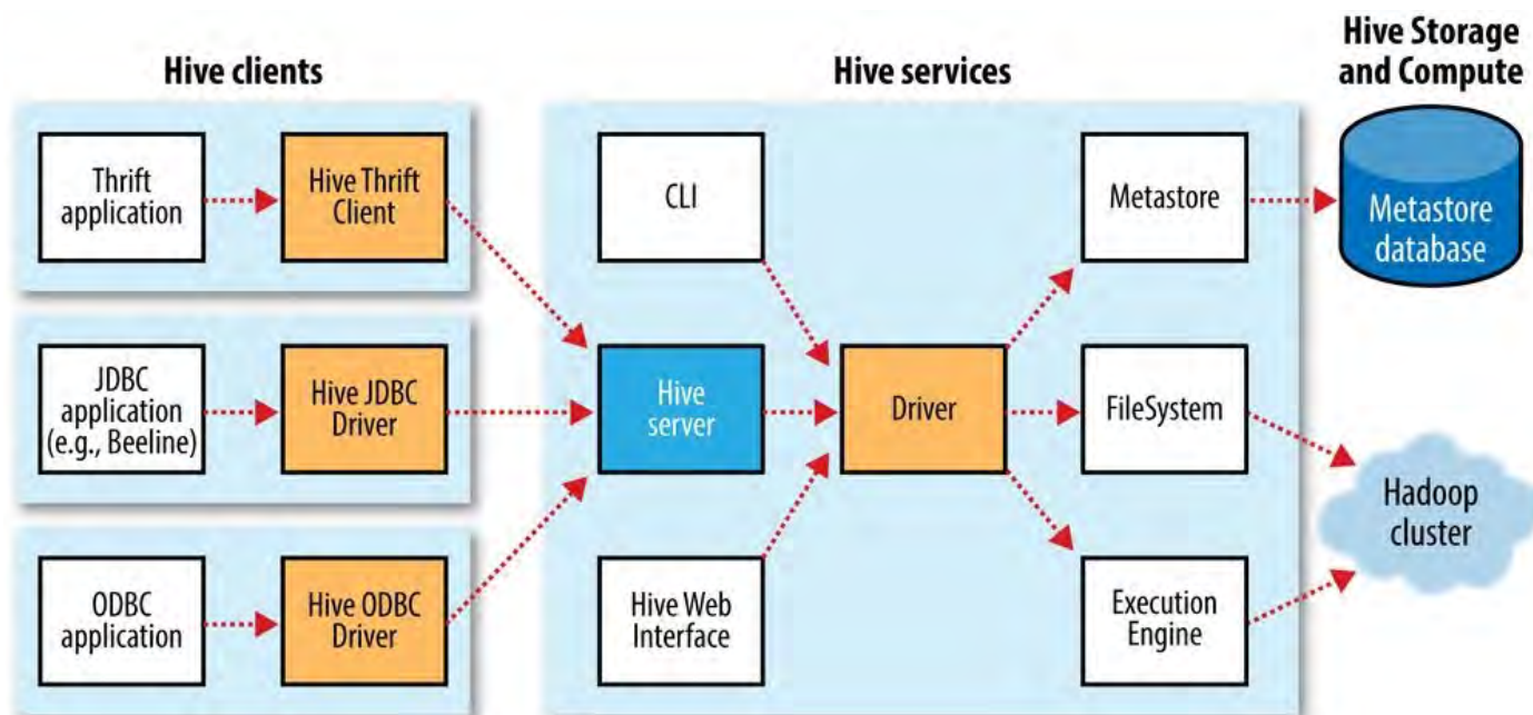
Figure 17-1. Hive architecture
