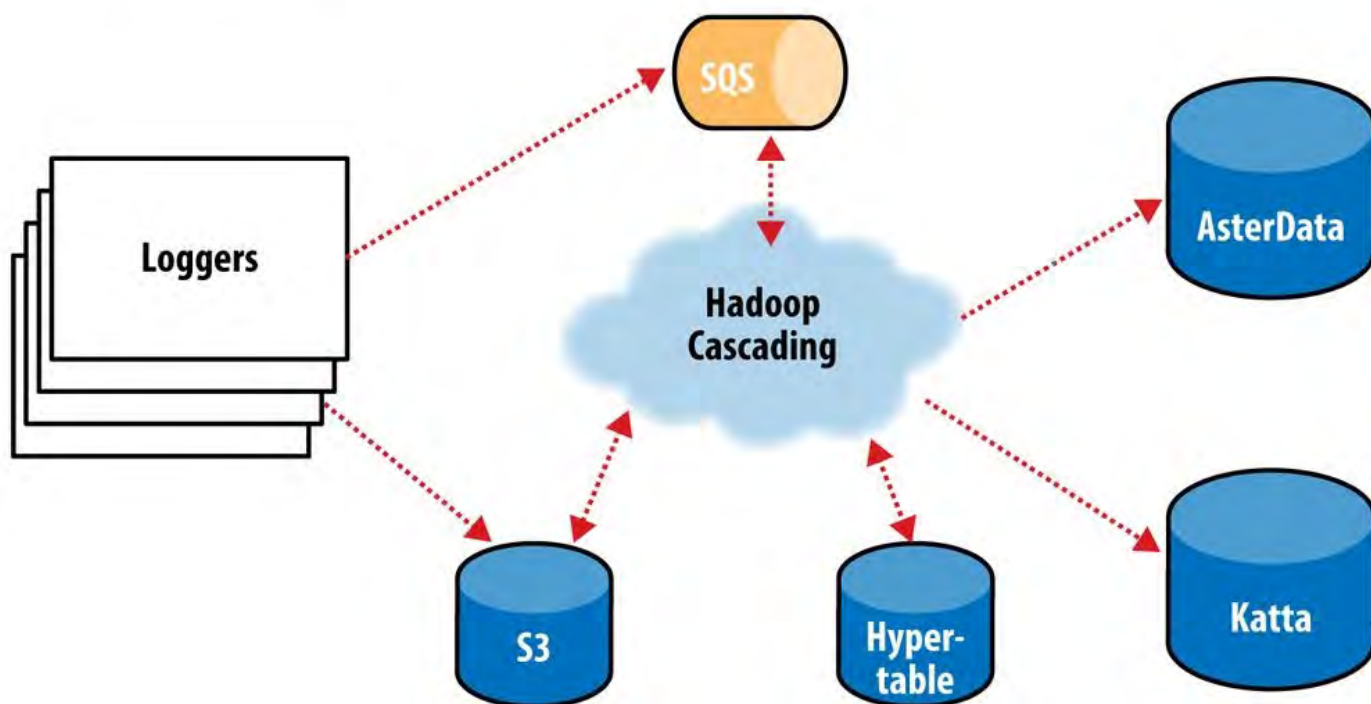
Figure 24-9. The ShareThis log processing pipeline
