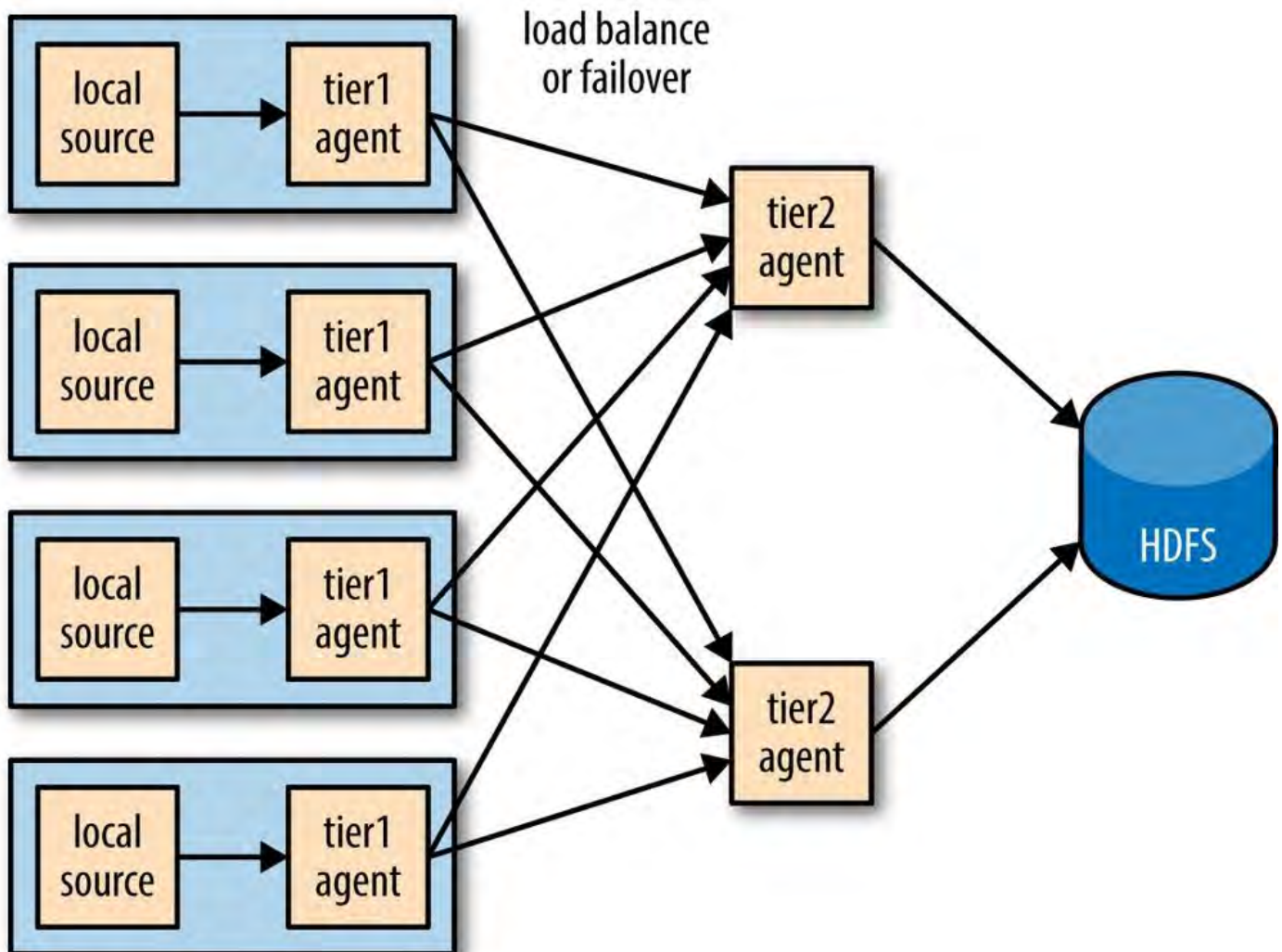
Figure 14-5. Using multiple sinks for load balancing or failover
