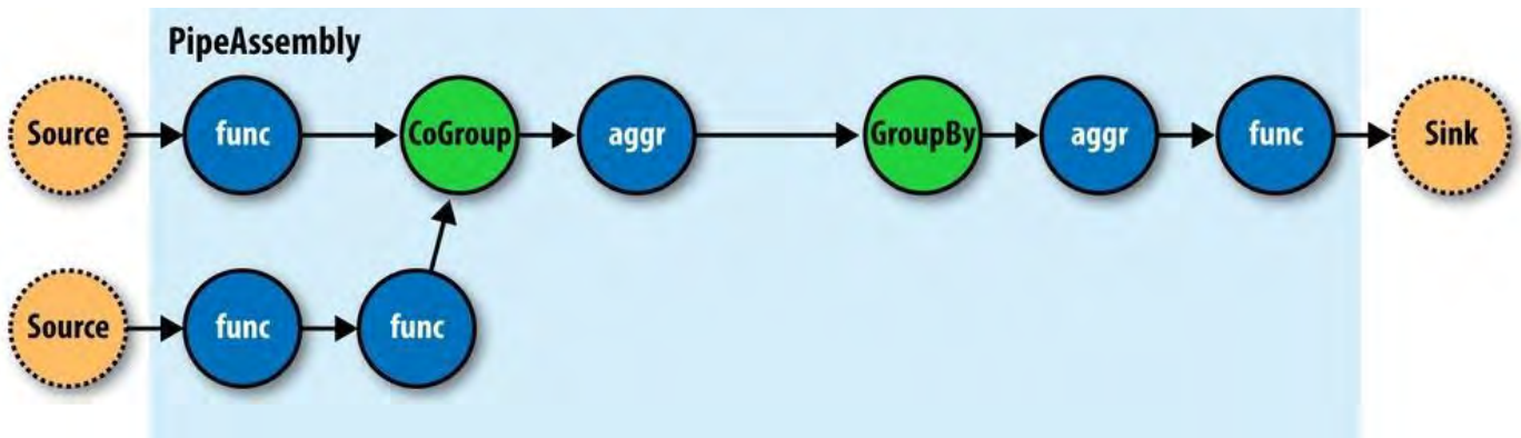
Figure 24-6. An assembly of operations
