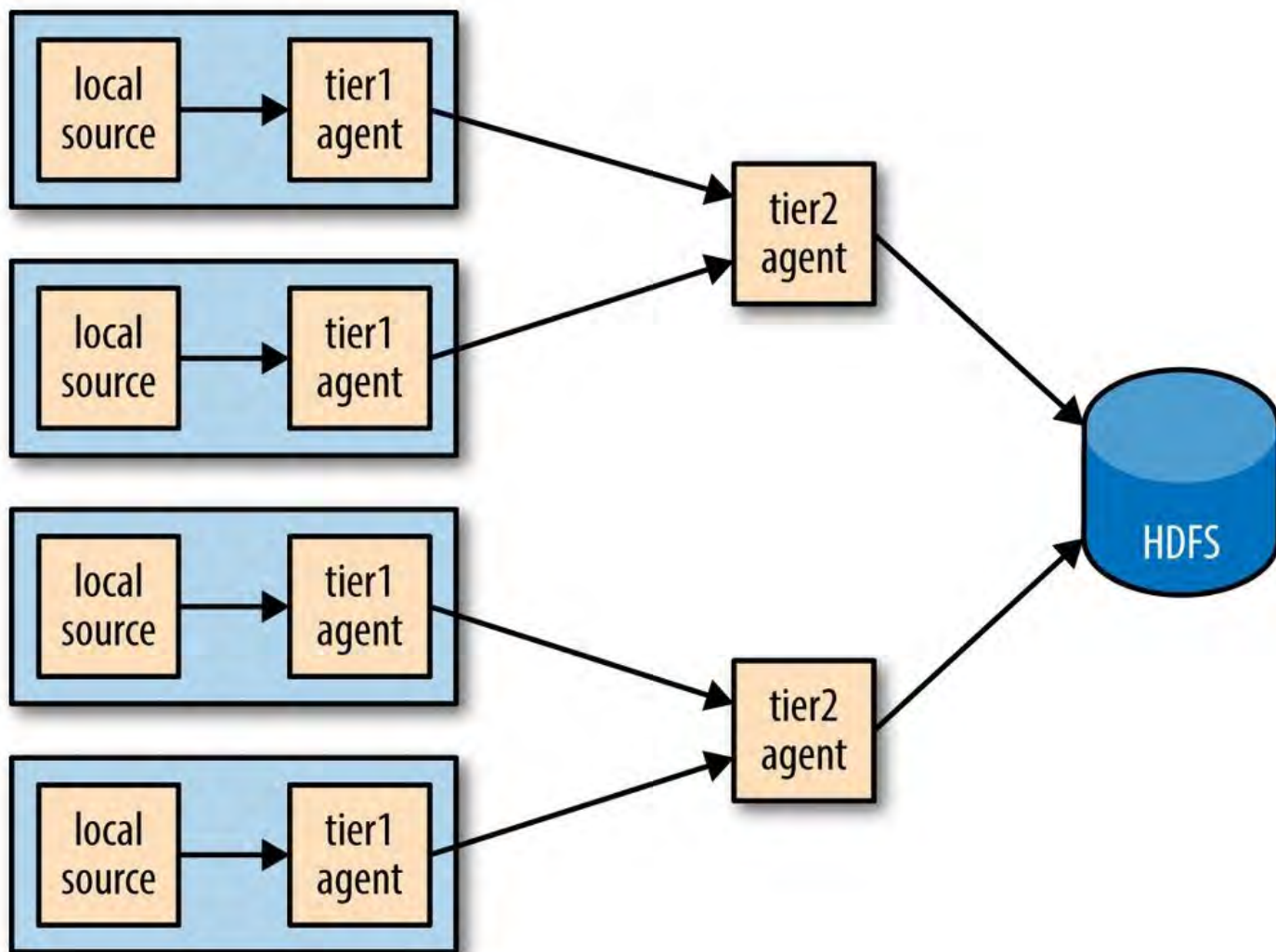
Figure 14-3. Using a second agent tier to aggregate Flume events from the first tier
