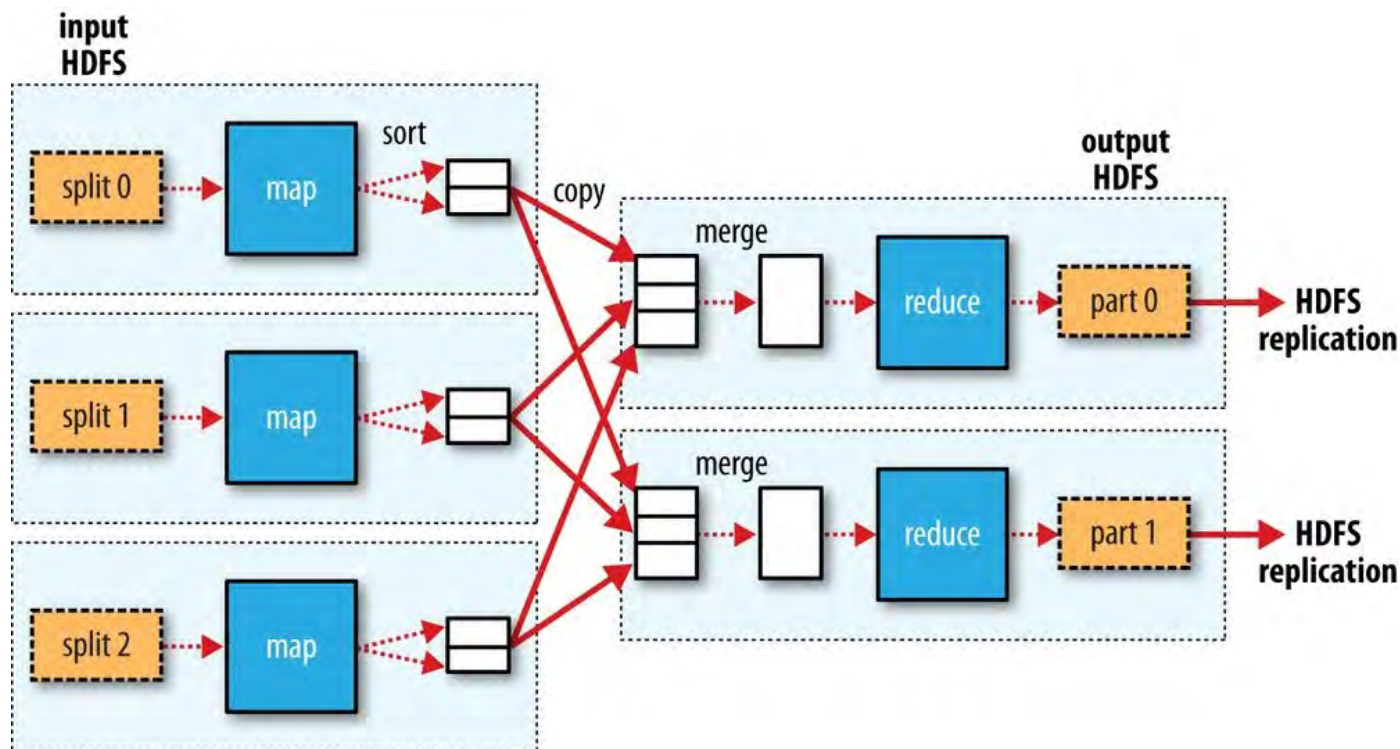
Figure 2-4. MapReduce data flow with multiple reduce tasks
