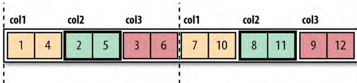
Figure 5-4. Row-oriented versus column-oriented storage
