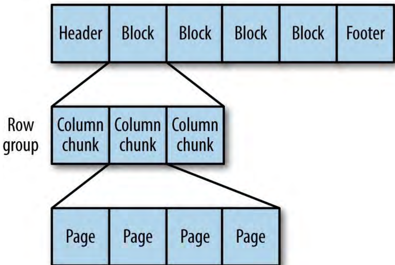
Figure 13-1. The internal structure of a Parquet file
