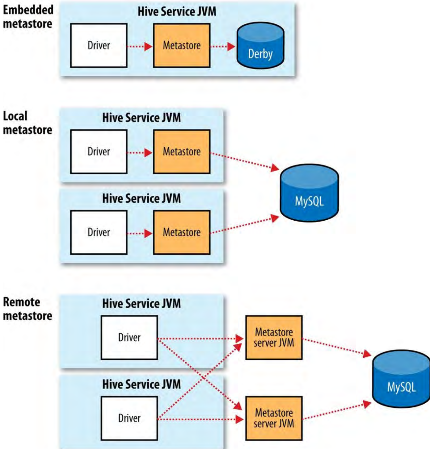
Figure 17-2. Metastore configurations
