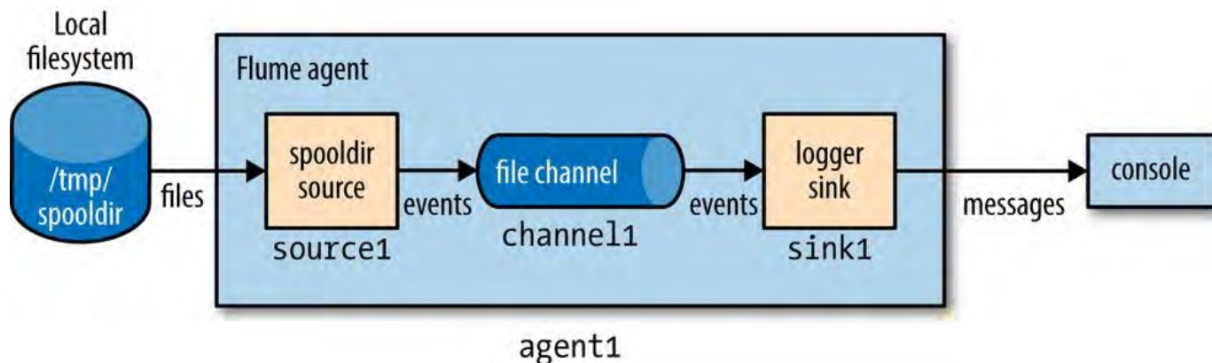
Figure 14-1. Flume agent with a spooling directory source and a logger sink connected by a file channel
