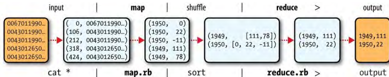
Figure 2-1. MapReduce logical data flow
