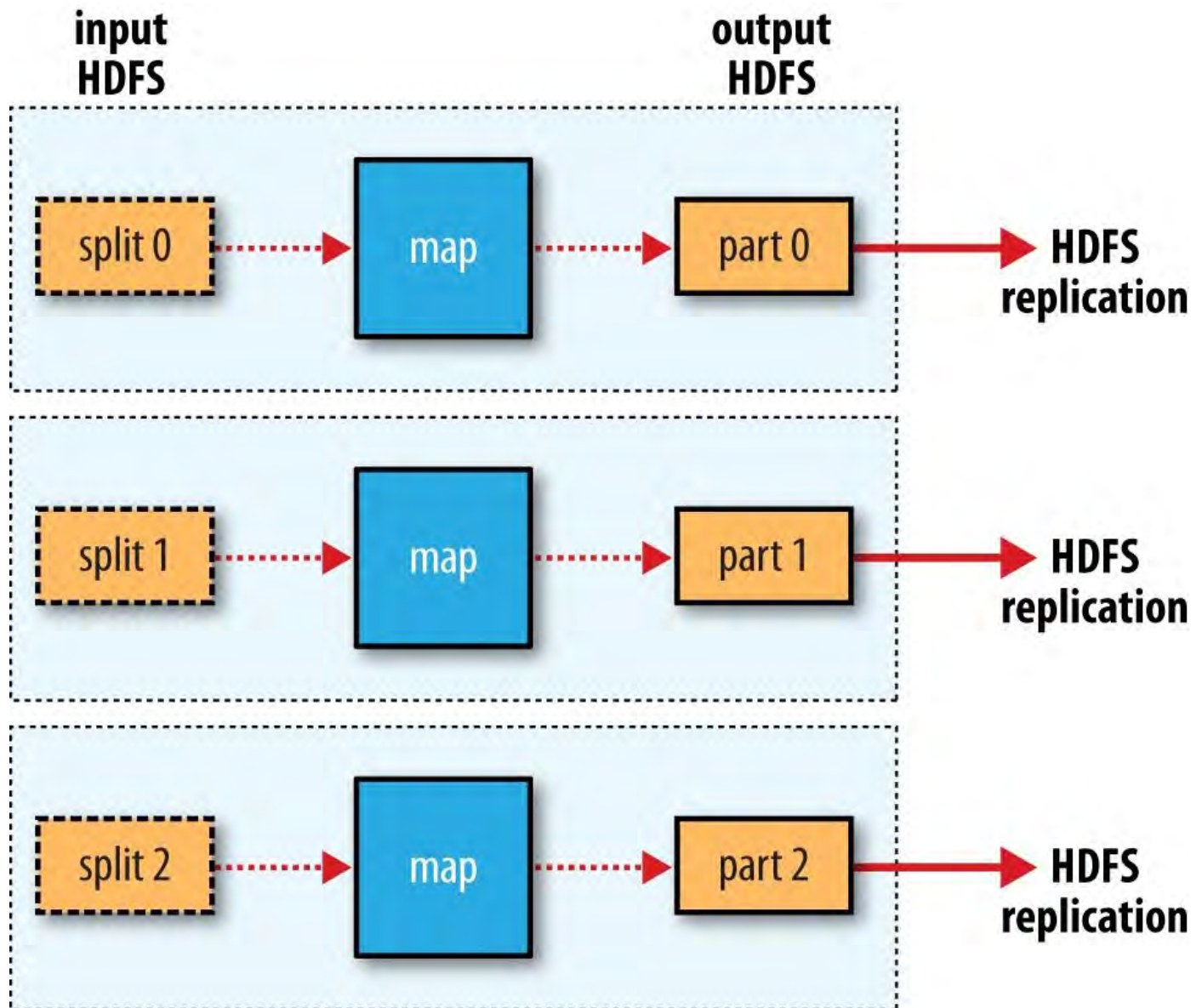
Figure 2-5. MapReduce data flow with no reduce tasks
