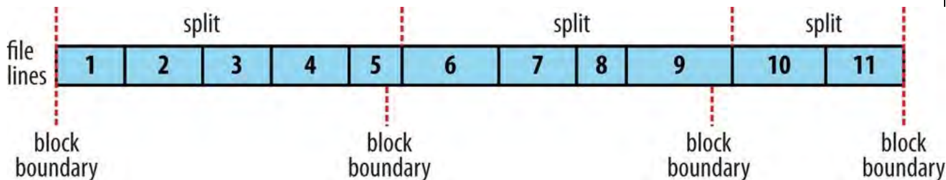
Figure 8-3. Logical records and HDFS blocks for TextInputFormat
