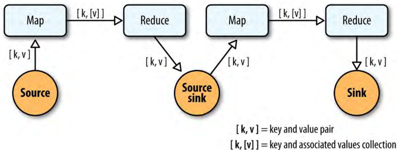
Figure 24-1. Counting and sorting in MapReduce
