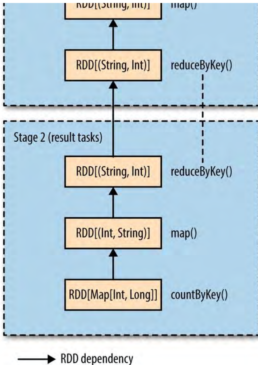
Figure 19-2. The stages and RDDs in a Spark job for calculating a histogram of word counts
