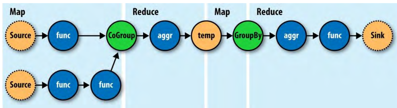
Figure 24-8. How a Flow translates to chained MapReduce jobs
