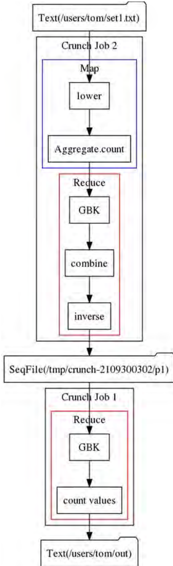
Figure 18-1. Plan diagram for a Crunch pipeline for calculating a histogram of word counts
