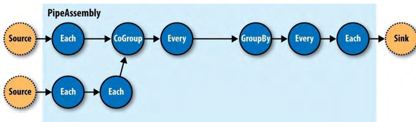
Figure 24-4. A simple PipeAssembly
