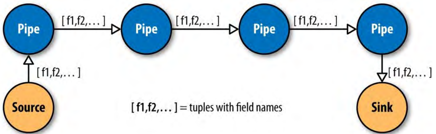
Figure 24-2. Pipes linked by fields and tuples
