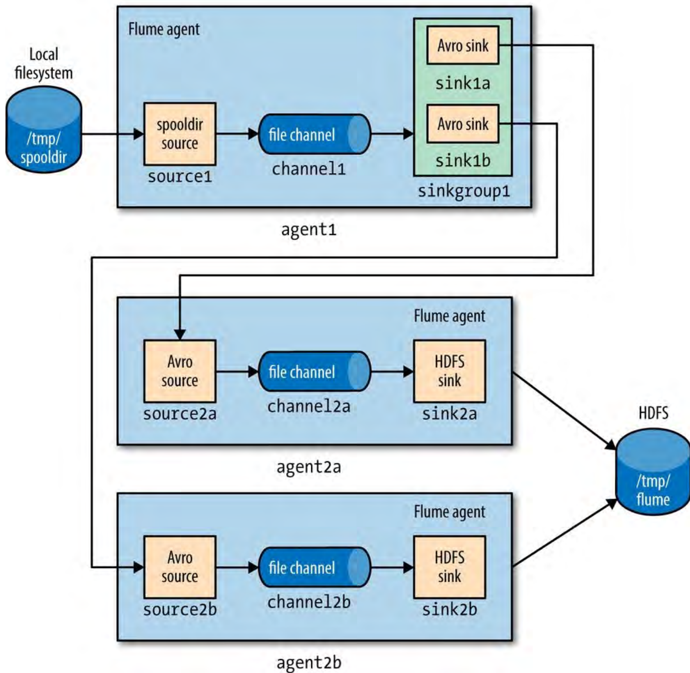
Figure 14-6. Load balancing between two agents
