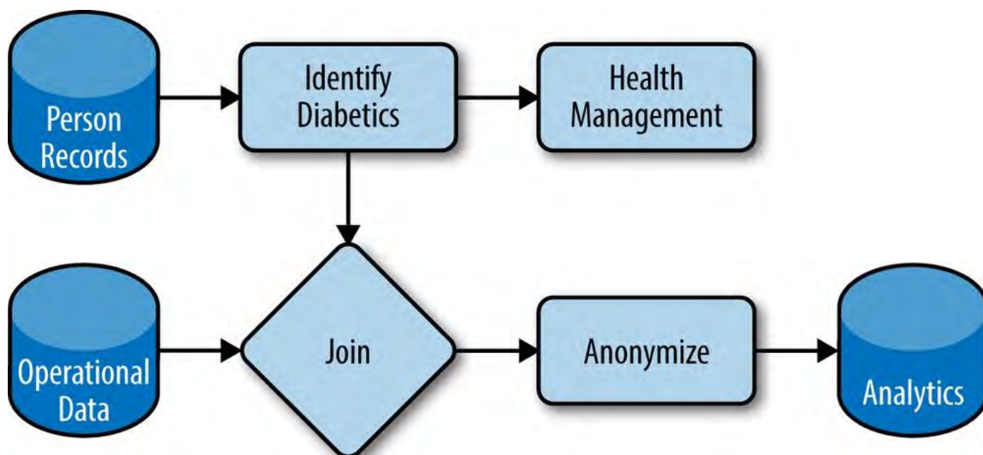
Figure 22-2. Composable datasets and functions
