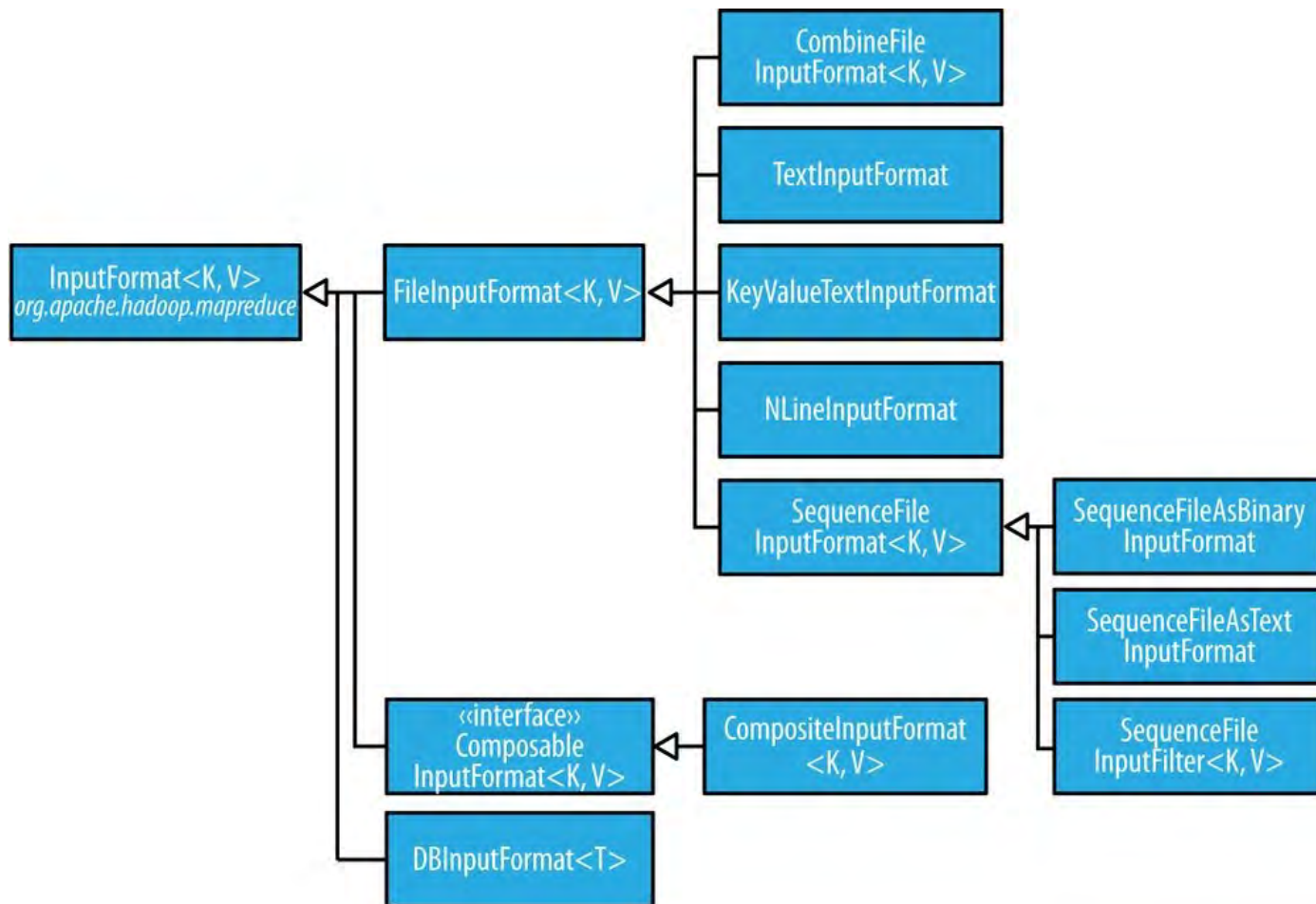
Figure 8-2. InputFormat class hierarchy
